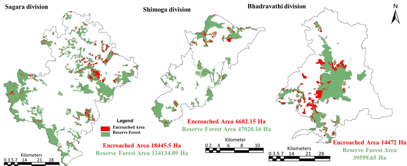
Fig. 7 Forest area encroachment across the divisions
