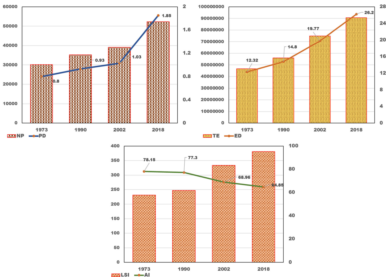
Fig. 5 Temporal pattern analysis through spatial metrics
