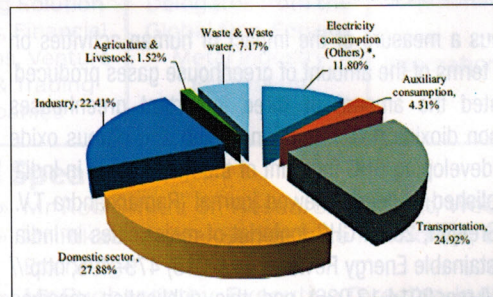
GHG footprint (carbon dioxide equivalent emissions, Gg) of Ahmedabad.
