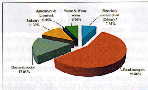
GHG footprint (carbon dioxide equivalent emissions, Gg) of Hyderabad.
