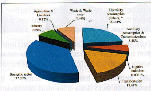
GHG footprint (carbon dioxide equivalent emissions, Gg) of Greater Mumbai.
