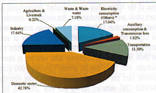
GHG footprint (carbon dioxide equivalent emissions, Gg) of Kolkata.
