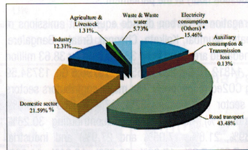
GHG footprint (carbon dioxide emissions, Gg) of Greater Bangalore.
