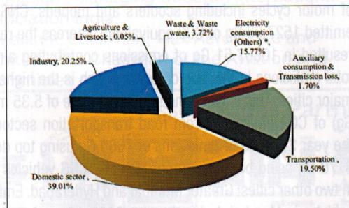
GHG footprint (carbon dioxide equivalent emissions, Gg) of Chennai in 2009-2010.
