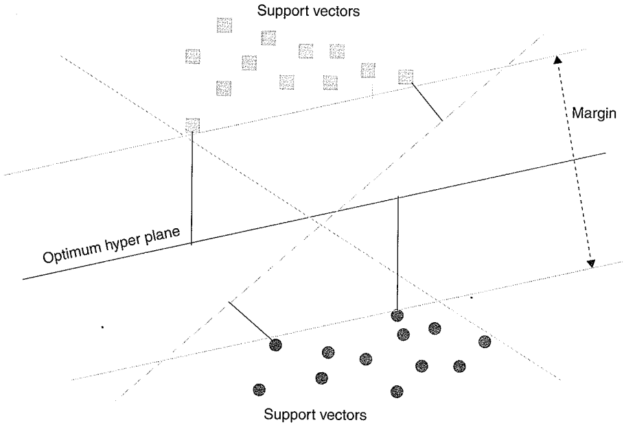
Fig. 1 Optimum hyper plane for linearly separable data with support vectors
