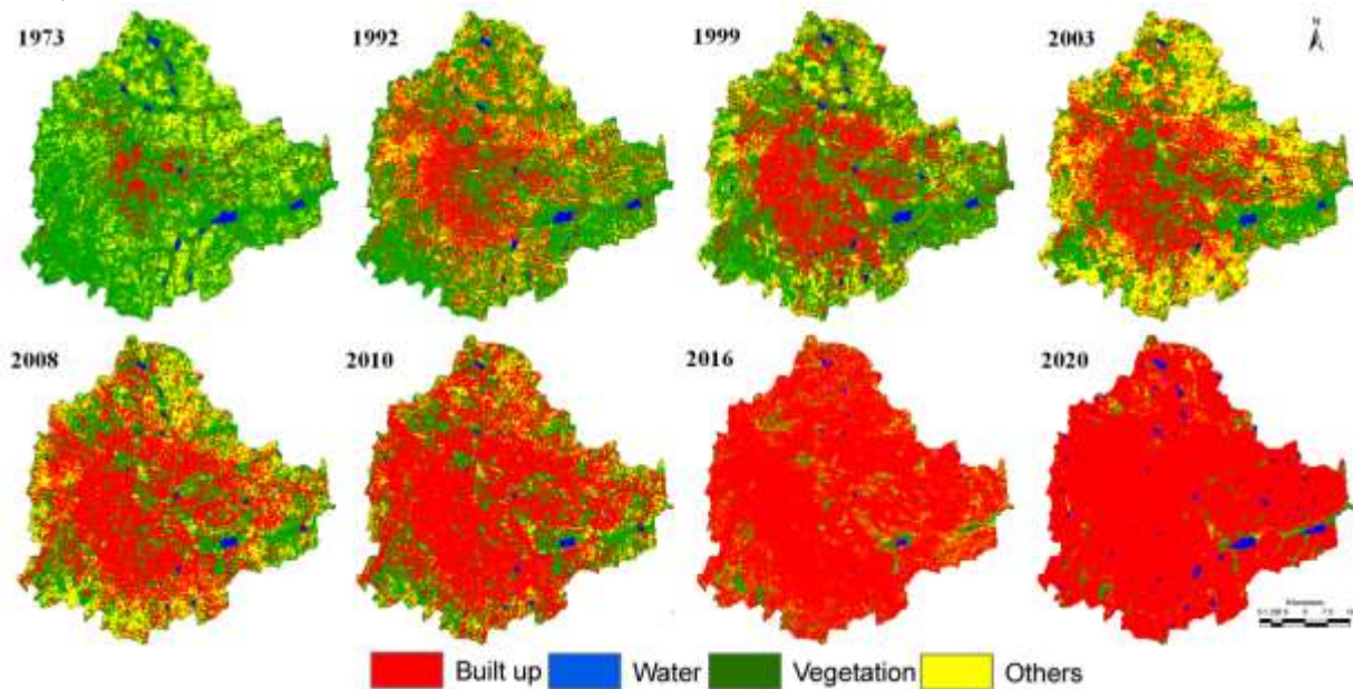
Fig. 1. Urban growth in Bangalore (based on temporal data acquired through space borne sensors)
