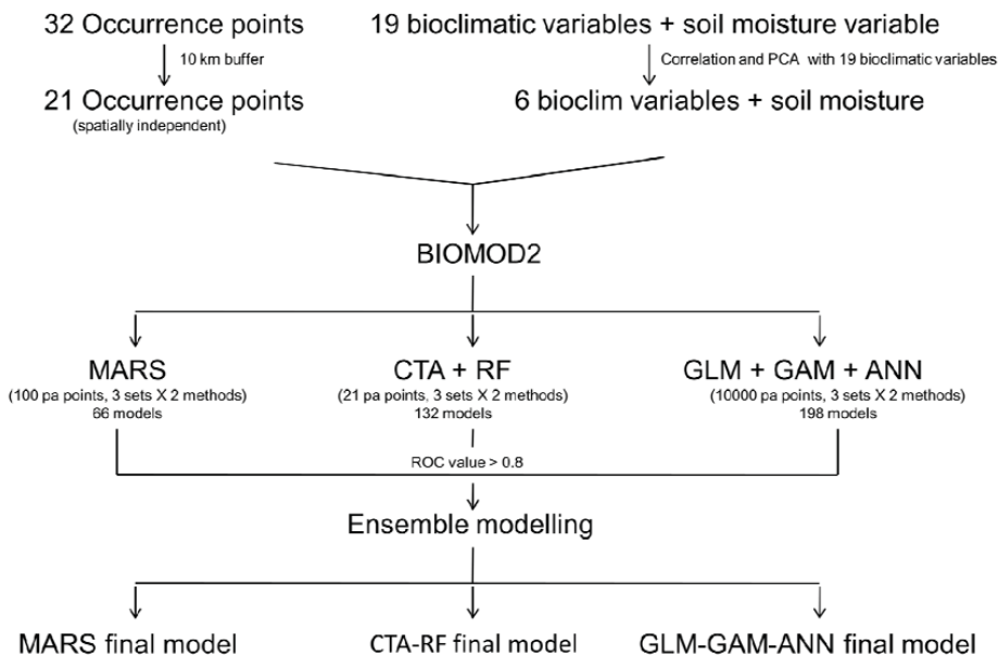
Figure 2. Modelling framework in BIOMOD2
