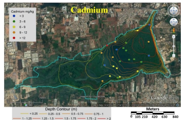
Fig. 5 Concentration of cadmium in sediment samples
