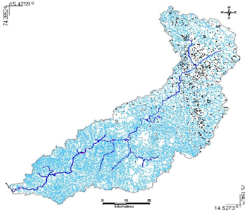
Figure 10: Drainage network of Bedthi River
