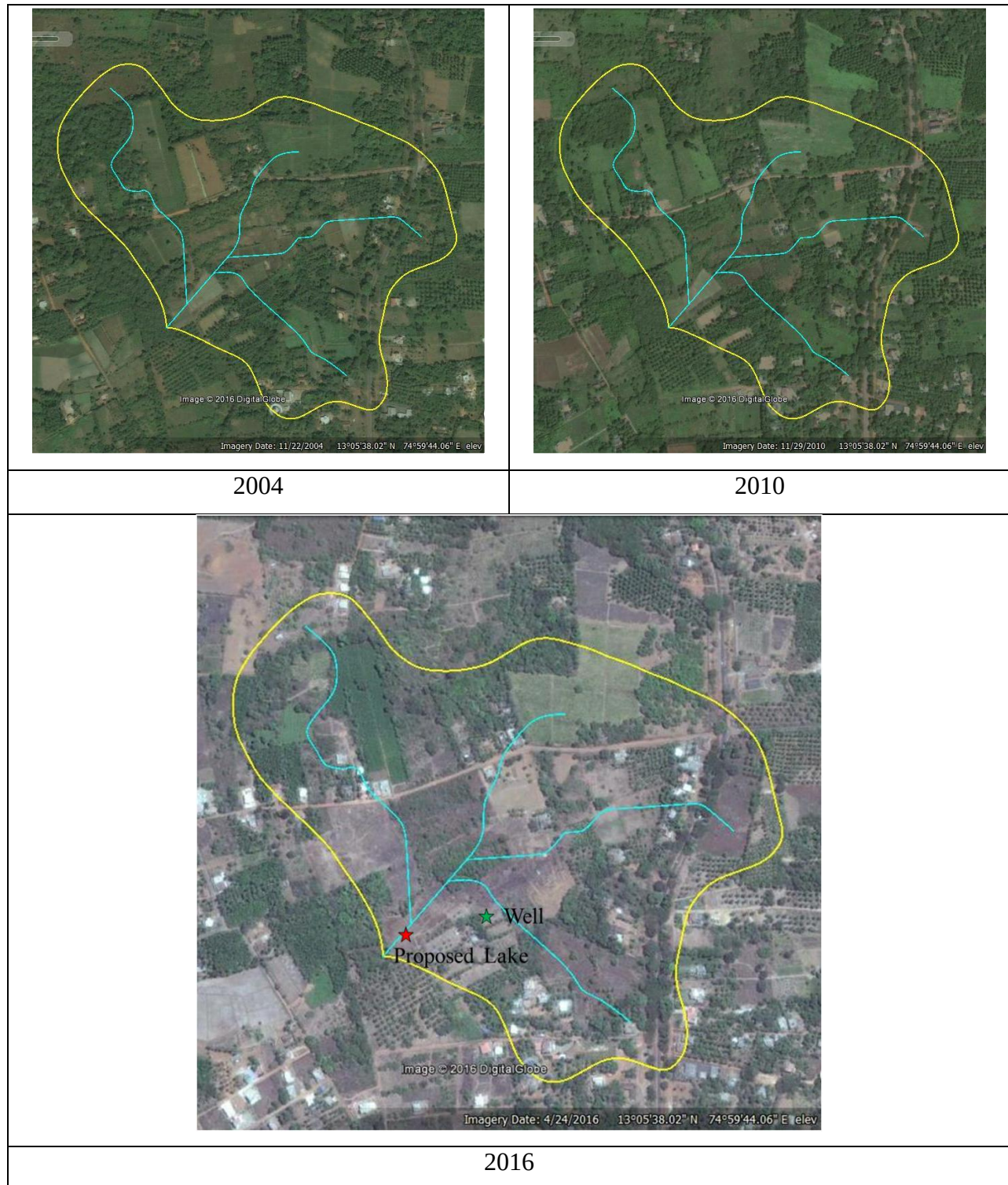
Figure 5: Landscape dynamics in the catchment.
