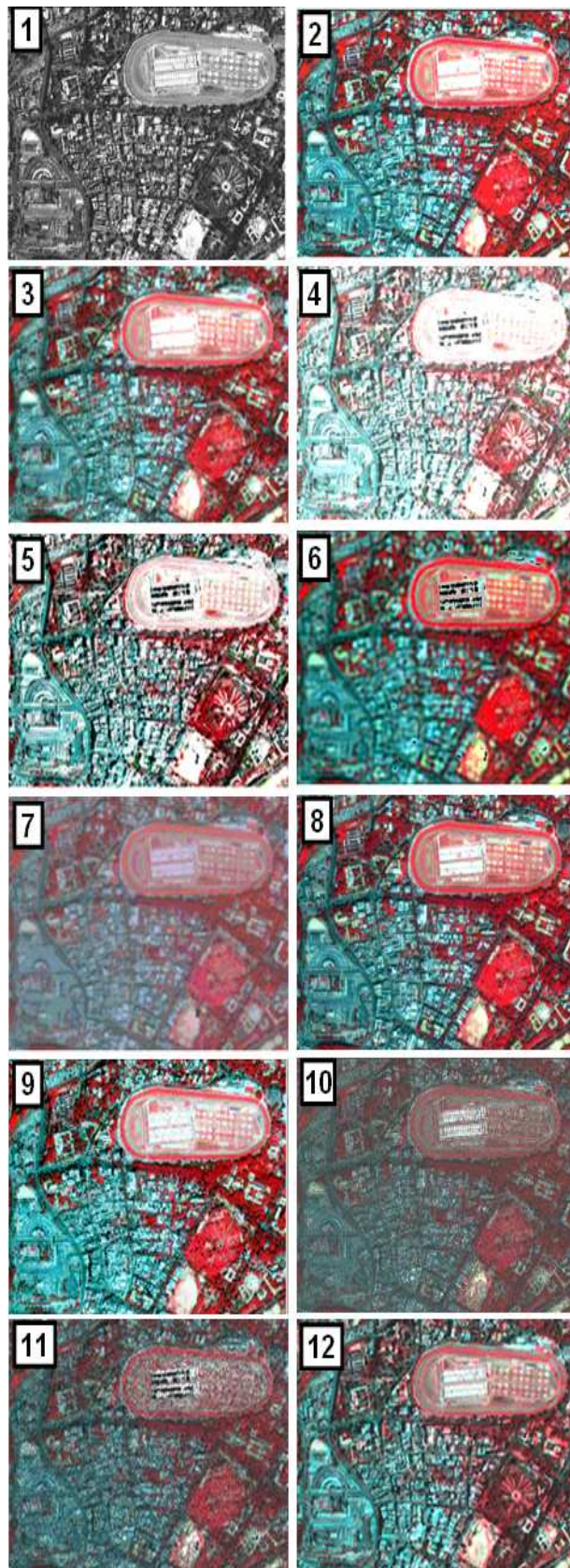
Figure 1. Original PAN image [1], FCC of the original LSR MS image (G-R-NIR) resampled at 1 m pixel size [2], Fusion through COS [3], LMVM [4], Modified IHS [5], FFT-IHS [6], GLP [7], LR [8], SF [9] Sparkle [10], SVHC [11] and SVR [12].
