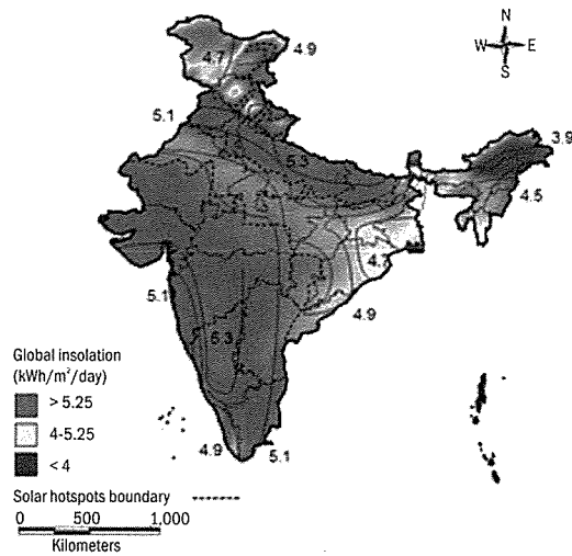
Figure 13: Annual average global insolation map of India showing the isohels and solar hotspots
