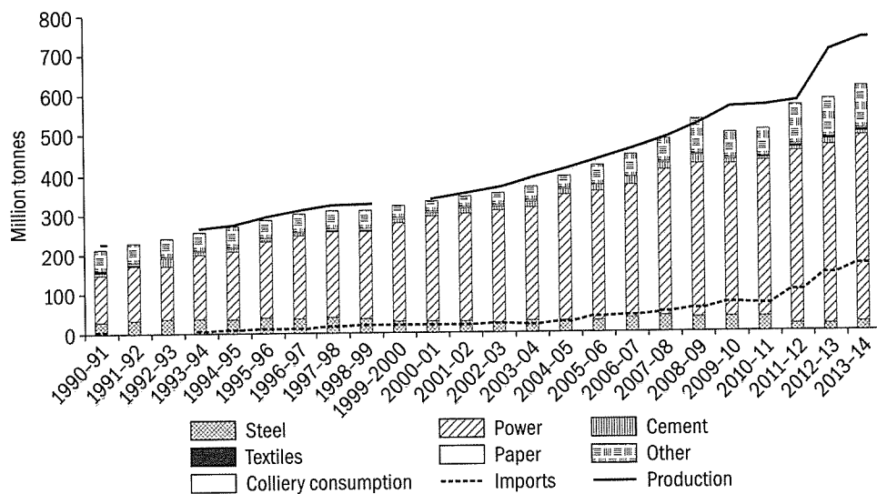
Figure 3: Temporal change in coal production, imports, and sector-wise consumption
