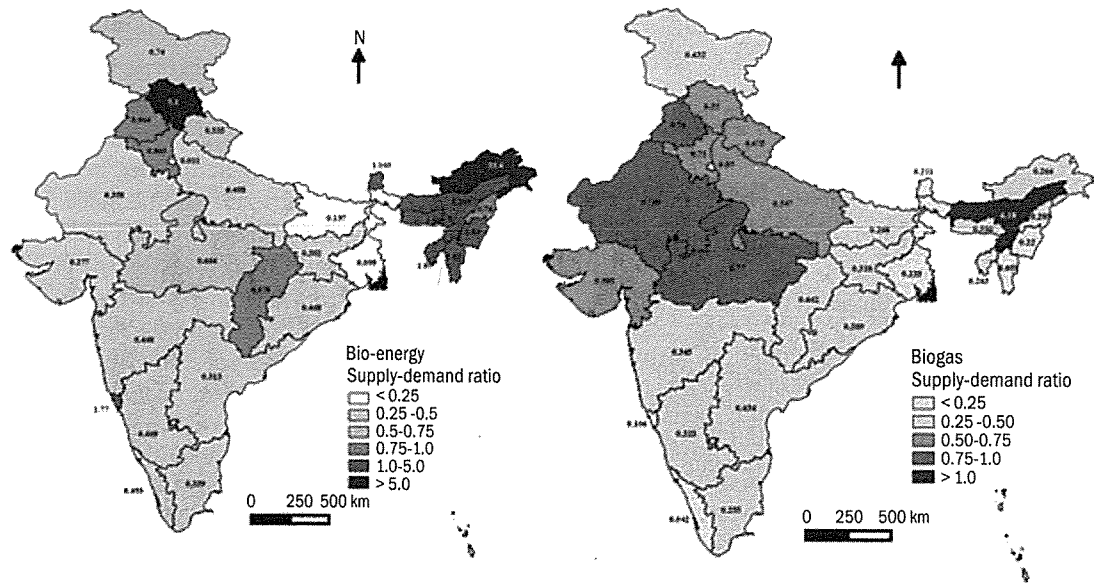
Figure 16: State-wise bioenergy and biogas status (supply/demand ratio)
