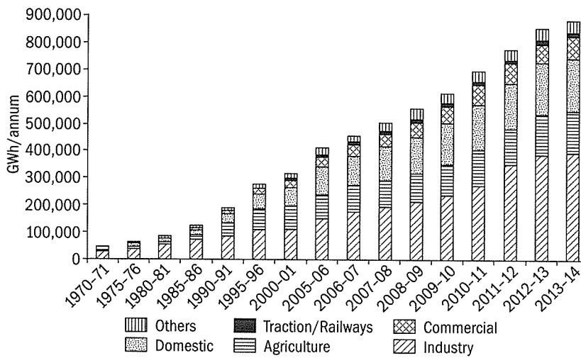
Figure 8: Sector-wise electricity consumption in India
