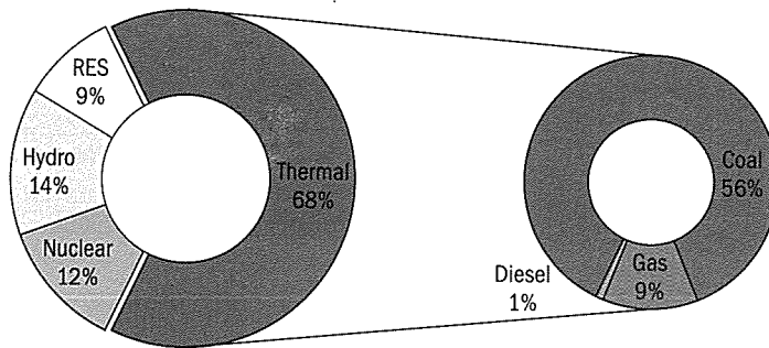
Figure 7: Share of energy sources in total installed capacity
