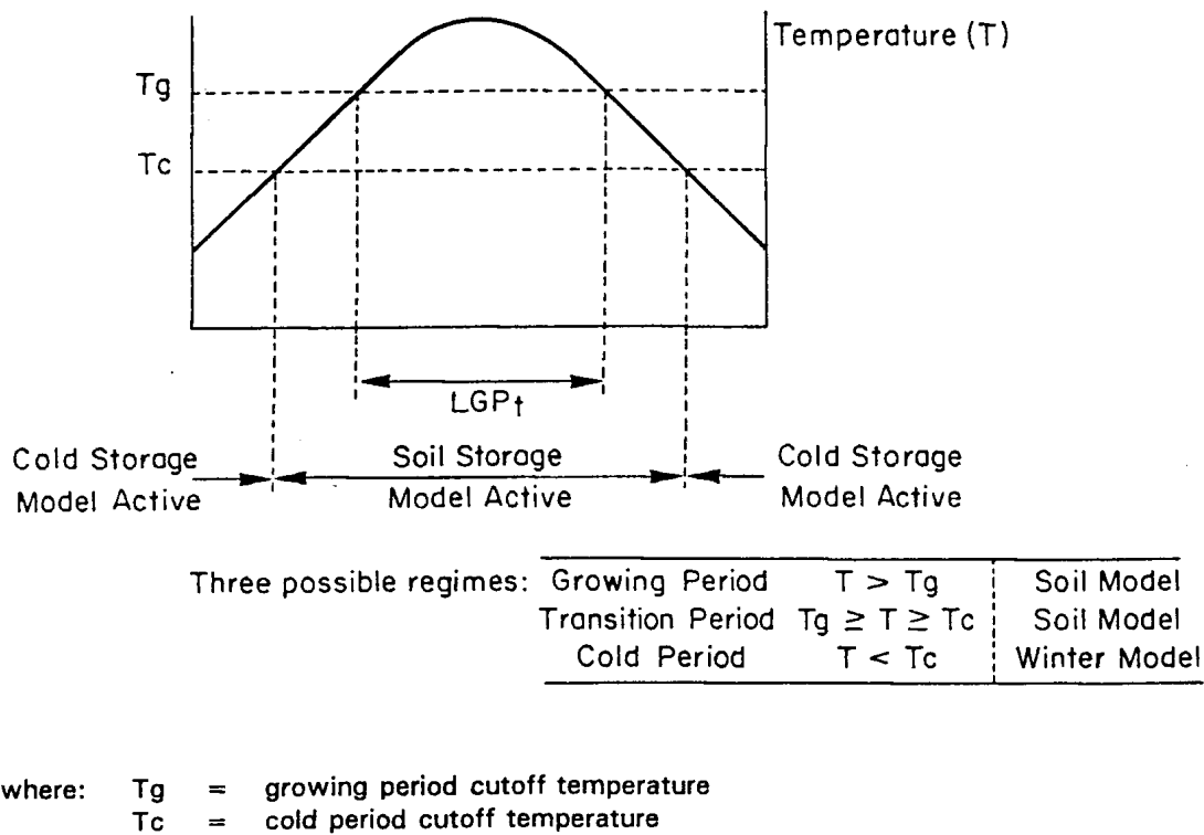
FIGURE 6 LGP and moisture balance models in China AEZ study
