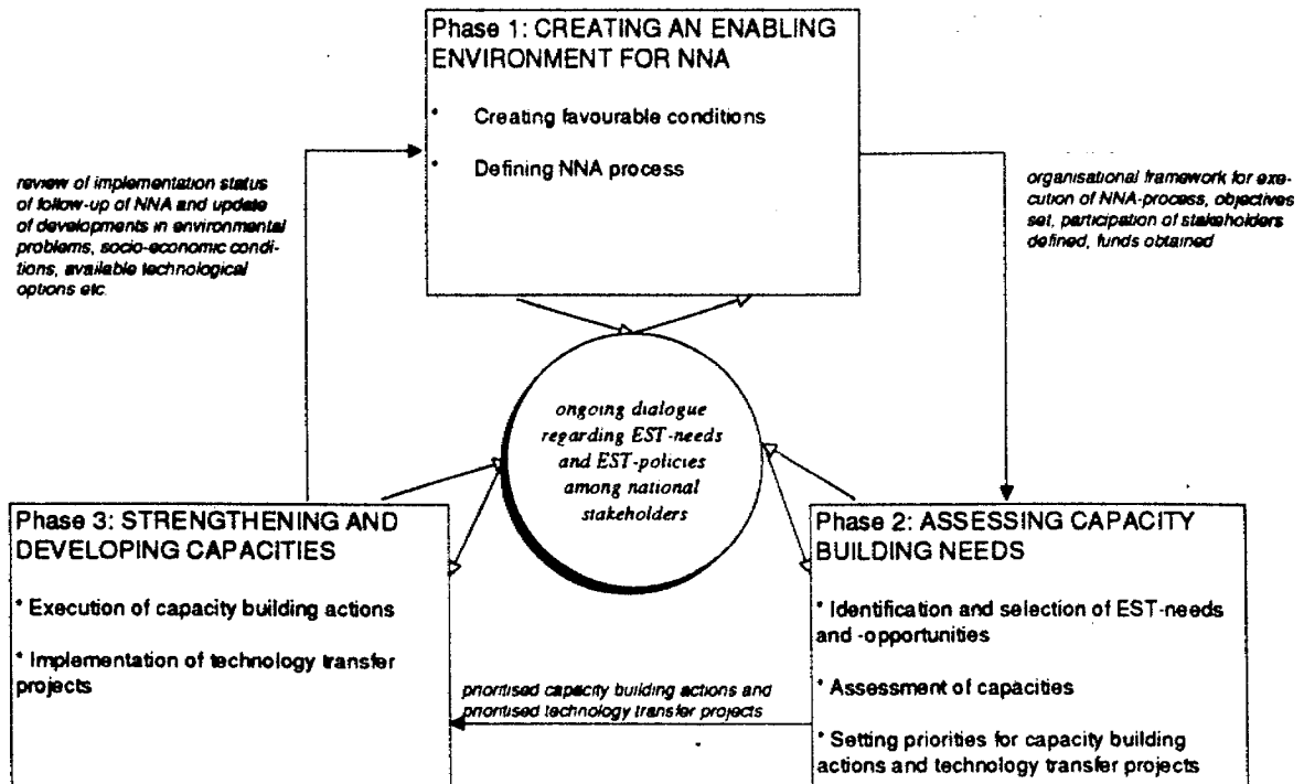
Figure 3: The NNA-process.
