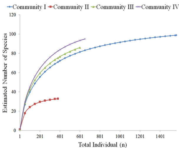
Figure 2 Individual based rarefaction curves for four identified shrub communities
