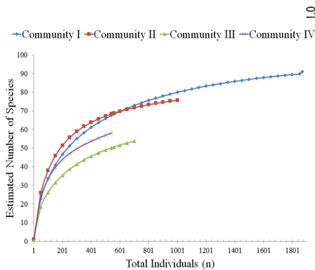
Figure 5 Individual based rarefaction curves for four identified communities in alpine meadows
