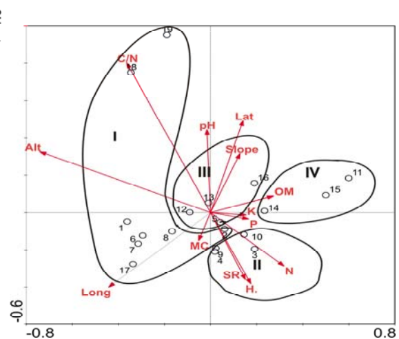
Figure 6 CCA ordination plot of sample and environmental variables for alpine meadow vegetation. Communities identified by cluster analysis are circled.
