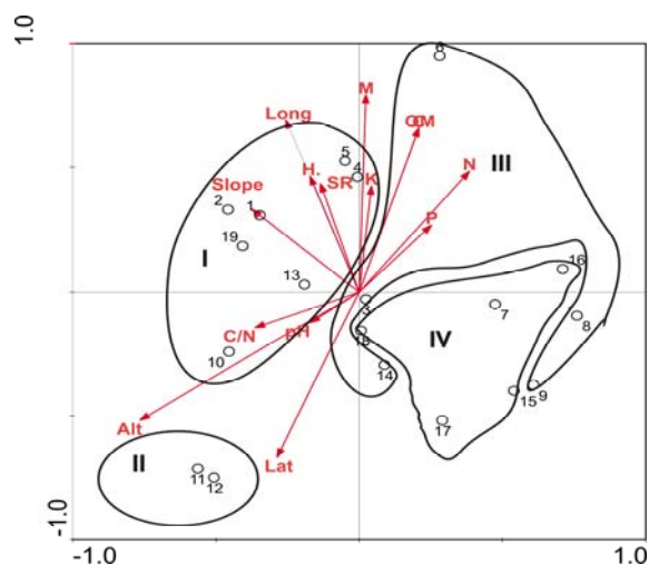
Figure 3 CCA ordination plot of samples and environmental variables in alpine shrub vegetation. Communities identified by cluster analysis are circled.
