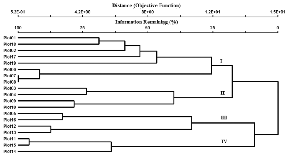
Figure 4 Dendrogram showing the different associations of meadows identified by the hierarchical agglomerative cluster analysis
