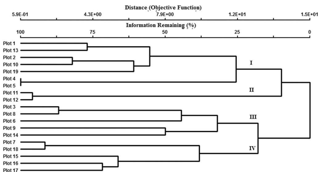
Figure 1 Dendrogram showing the different associations of shrubs identified by the hierarchical agglomerative cluster analysis
