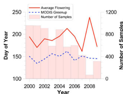
Fig. 2 Solid lines Average flowering time estimated from herbarium records, dotted lines MODIS-derived greenup estimates. Bars Number of herbarium samples collected in flower each year
