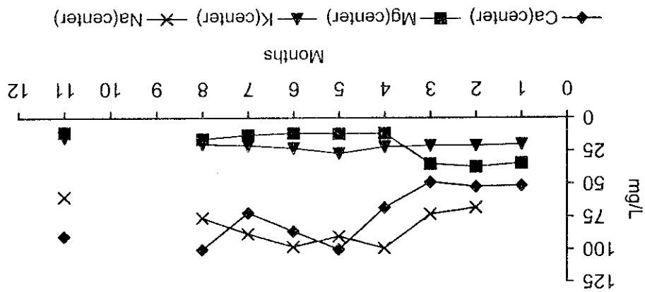
Figure 11.9: Ca, Mg, K, Na
