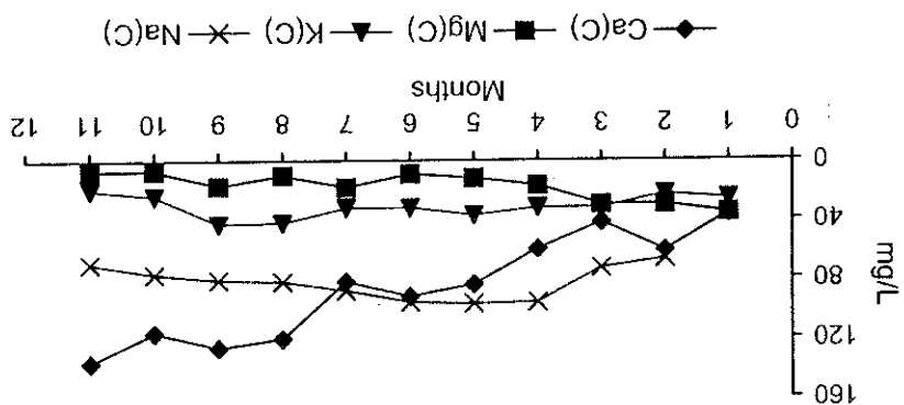
Figure 13.12: Ca, Mg, K, Na
