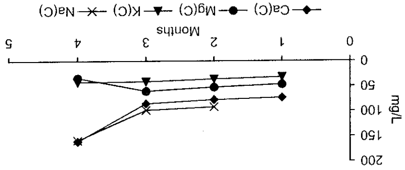
Figure 12.9: Ca, Mg, K, Na (C)
