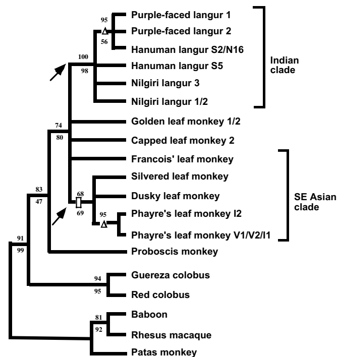
Fig. 3. Prm1 phylogeny of the langurs and leaf monkeys. This is a strict consensus of three equally parsimonious trees (length = 90). The numbers above and below the branches indicate bootstrap support for the MP and ME trees, respectively. Arrows indicate the species groups that were always monophyletic irrespective of the method used for tree building. The symbols “□” and “Δ” indicate shared unique amino acid replacement and shared unique amino acid deletion, respectively. Identical sequences are indicated by “/”. Refer to Table 2 for sample information and abbreviations. Prm1 gene tree supports the clustering of Nilgiri and purple-faced langurs with Hanuman langur with high bootstrap support (Fig. 3). Dusky, silvered, and Phayre’s leaf monkeys also form a clade (but with low bootstrap support). However, it is interesting to note that they share one unique amino acid replacement in the protamine P1 protein sequences (Fig. 4). The topology of the ME tree
