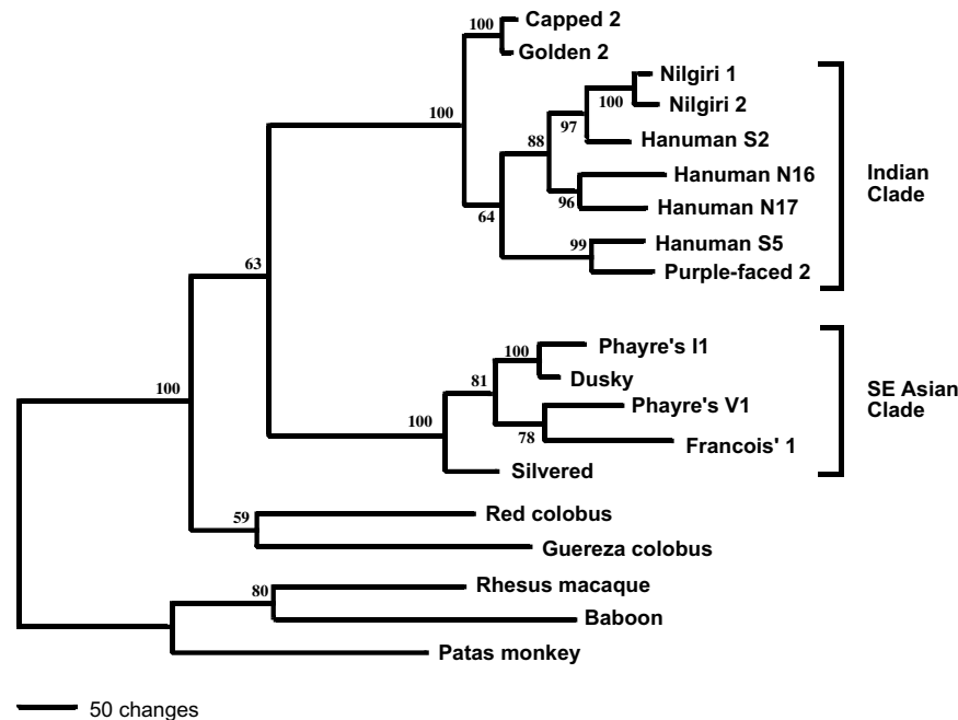
Fig. 2. The Cyt-b MP tree (length = 3063). Numbers above the branches indicate bootstrap support from 1000 replications with 10 random stepwise additions. The same overall tree topology (see text for details) was obtained by ML option (HKY85 G+I, –clock, -\ln L = 6696.4978 ). In the case of minimum evolution tree (HKY85 G+I) there were minor rearrangements of taxa within the Indian clade and the SE Asian clade (see text). The bootstrap support for various nodes in the minimum evolution tree (not shown) was similar to the parsimony bootstrap values.
