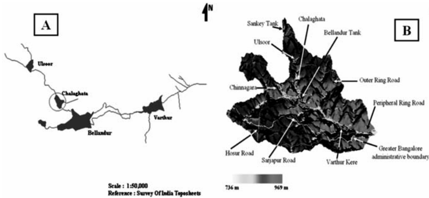
Figure 13.1: Ulsoor-Bellandur-Varthur (a) drainage network (b) lakes overlaid on 10 m DEM showing their missing interconnectivity
