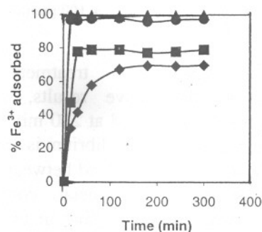
Fig. 4—Percentage biosorption of Fe(III) from solution at different metal concentration (▲ 10 ppm; ● 20 ppm; ■ 50 ppm; ◆ 100 ppm), pH 2.5, by 10 gL -1 bgh as related to the time of contact at 120 rpm
