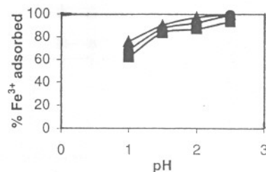
Fig. 3—Effect of pH on the biosorption of Fe(III) at different metal concentrations (▲ 10 ppm; ● 20 ppm; ■ 50 ppm), by 10 gL -1 at 120 rpm with equilibrium time of 200 min
