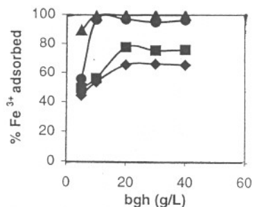
Fig. 5—Effect of quantity of bgh biomass on biosorption of Fe(III) from solutions at different metal concentrations (▲ 10 ppm; ● 20 ppm; ■ 50 ppm; ◆ 100 ppm), pH 2.5 for contact time of 200 min at 120 rpm
