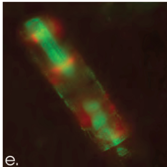
Figure 5. Intense red-fluorescing chlorophyllinite [fossil chlorophyll] preserved in association with green fluorescing diatom oils directly within diatom frustule [width 10 \mu\text{m} ]; imaged using a scan of 363 nm excitation, with 510 \pm 40 nm, 570 nm, and then >665 nm emission. (Reprinted, with permission, from ref 110. Copyright 2001, Elsevier, Amsterdam, The Netherlands.)
